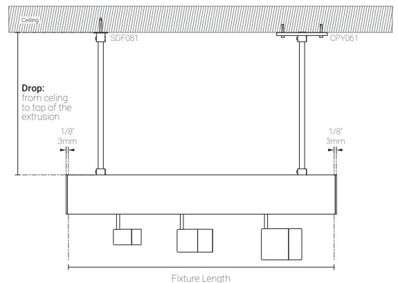
Fixture installed
