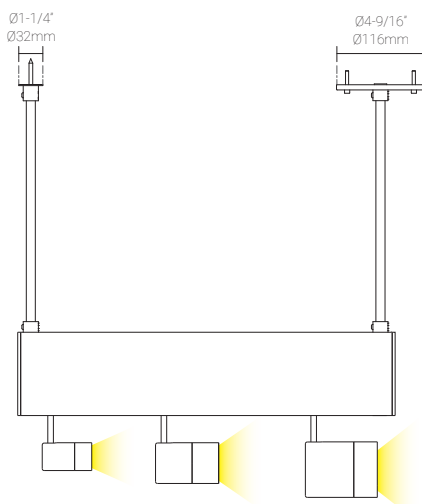
Mounting Dimensions
