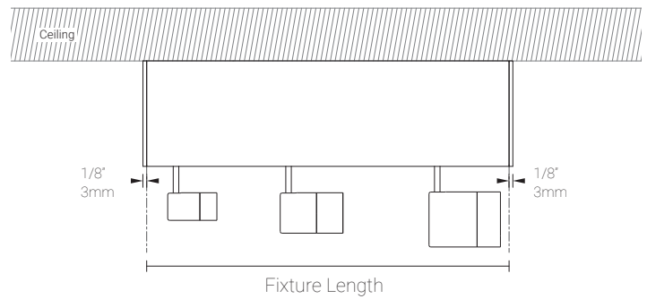
Fixture installed - Front
