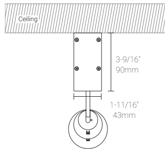
Fixture installed - Side
