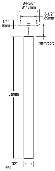
Shown with C3 canopy
