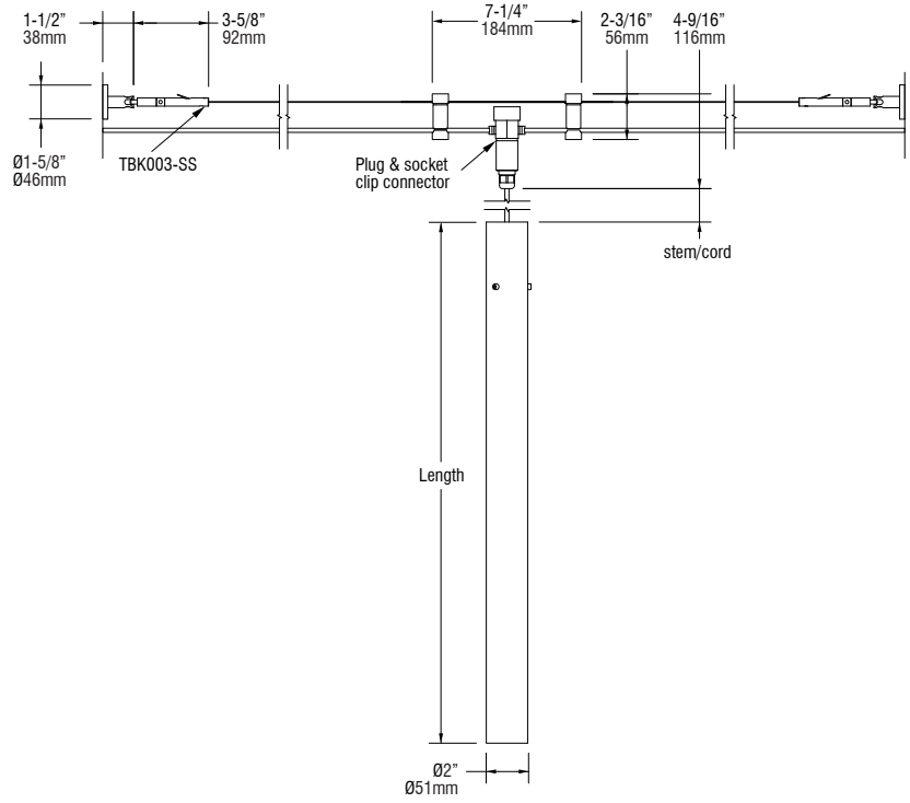
Shown with Plug & Socket Clip Connector with Turn Buckle
