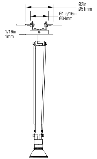
C21 2" (50.8mm) x 1/16" (1.59mm) with spring mount
