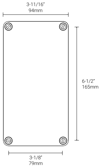
Back Box
