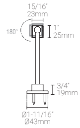
Fixture
