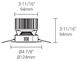
Fixture
