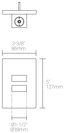
Fixture Top & Front View
