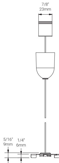
Cable Suspension Kit: Side View
