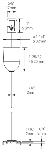
Cable Suspension Kit
