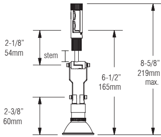
Fixture
