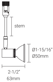
Fixture
